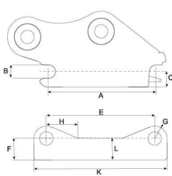
Dimensions and tolerance table
